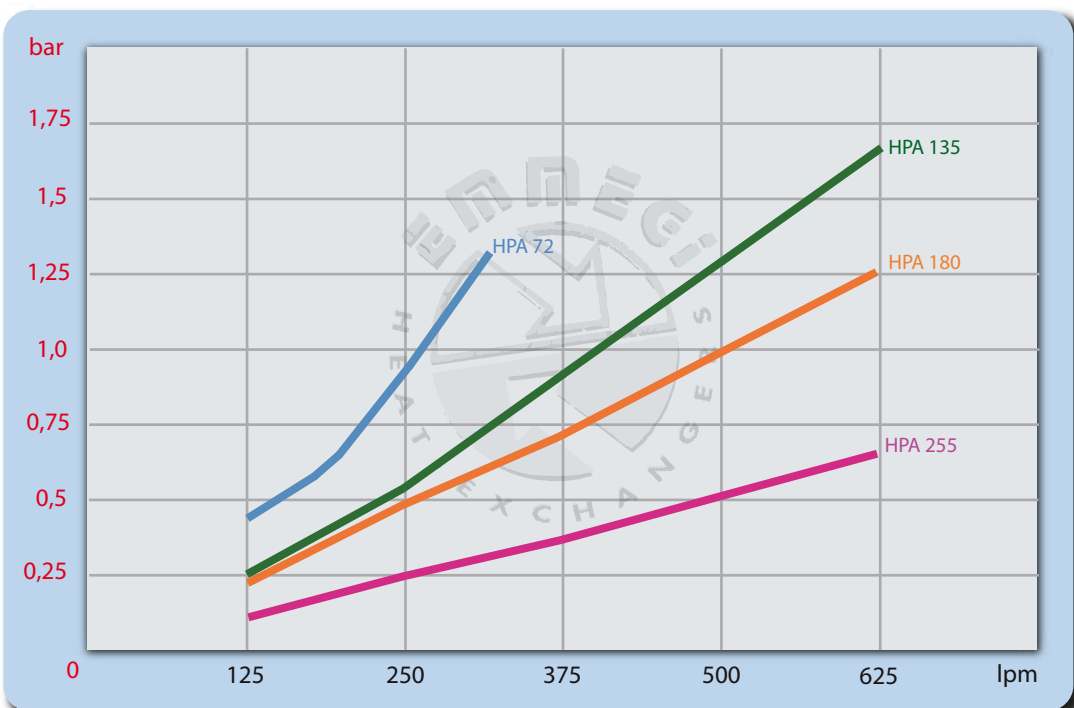
Pressure drop with oil ISO VG 32 @ 50°C
